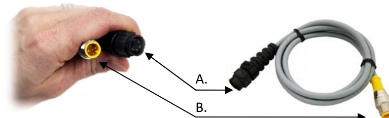
A. 5-pin Female Switchcraft Connector B. 5-pin Male M12 Connector
